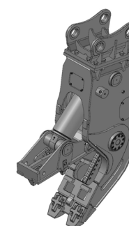
FP-V Series Fixed Pulverizer
