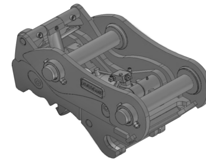
EQC-D Series Coupler (Dual locking)
