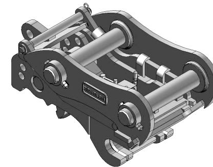
EQC-S Series Coupler (Single lock)
