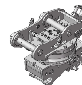
ERS-E Rotating coupler Series
